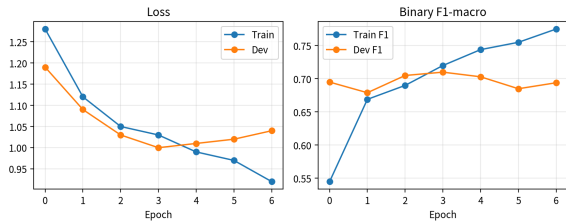
Figure 4: Training curves for loss (left) and binary macro-F1 (right).
