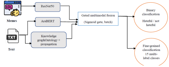
Figure 2: Overview of the multimodal architecture.
