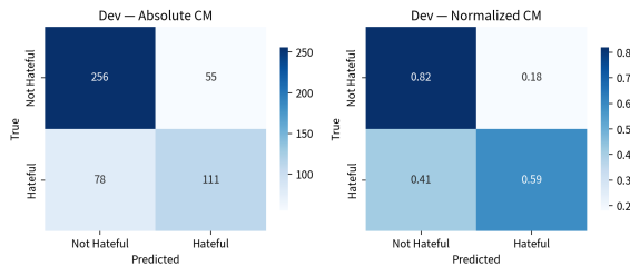
Figure 3: Binary confusion matrices on the development set (left: absolute counts; right: row-normalized).
