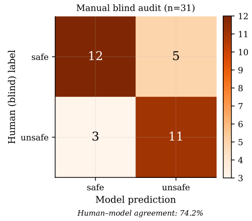
Figure 4: Confusion matrix from the blind manual audit ( n=31 ).
