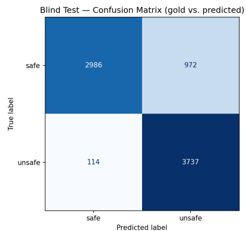
Figure 5: Confusion matrix on the full blind test set (n=7,809).
