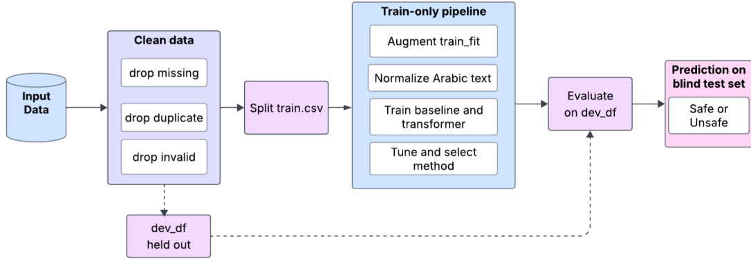
Figure 1: Leakage-controlled data flow: train.csv is split three ways; dev is used exactly once.
