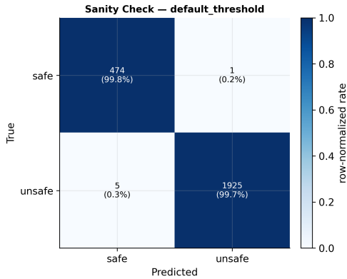
Figure 3: Confusion matrix on dev_with_label.csv (sanity check only; see Table 3 for the held-out result).
