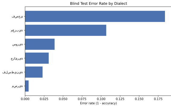
Figure 6: Blind test error rate by dialect.
