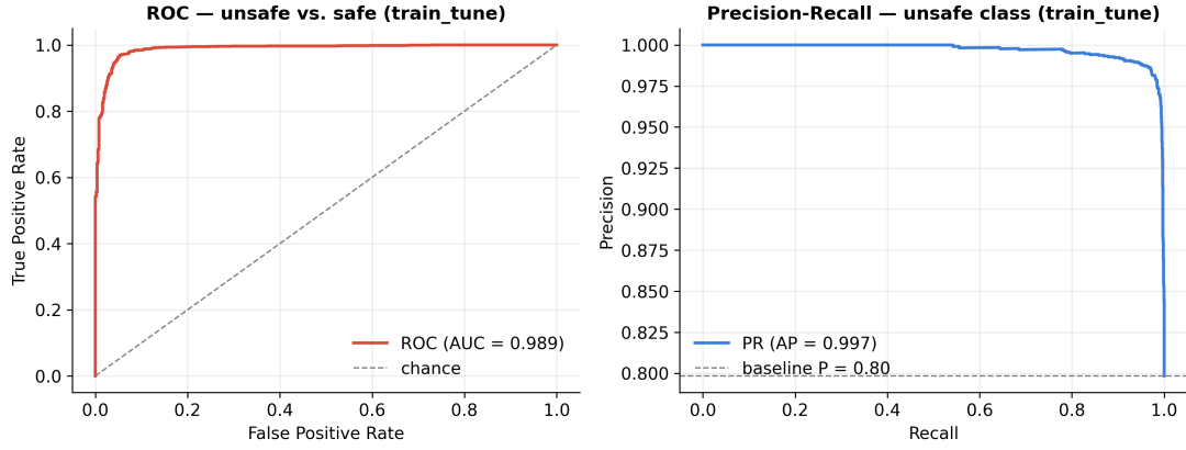
Figure 2: ROC and Precision-Recall curves for MARBERTv2 on train_tune.
