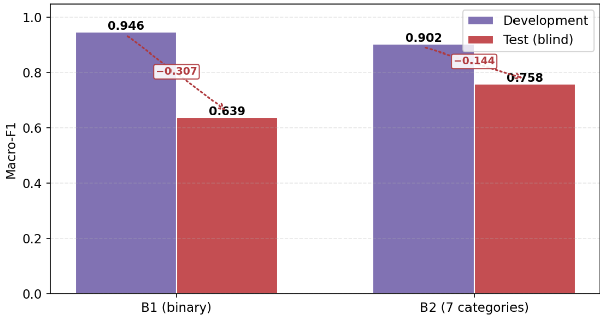
Figure 6: Generalization gap.
