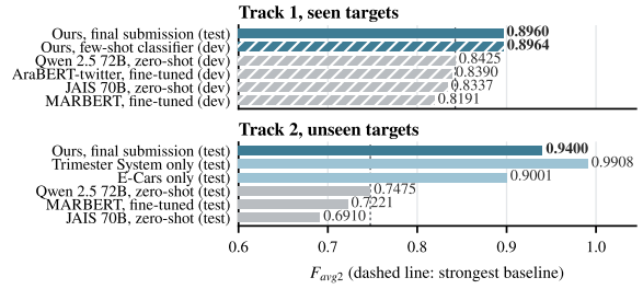
Figure 1: Official F_{\text{avg2}} of our final submissions (dark blue), our score on each Track 2 target (light blue) and the organizers’ baselines (grey). Hatched bars are development-set scores, solid bars test-set scores.
