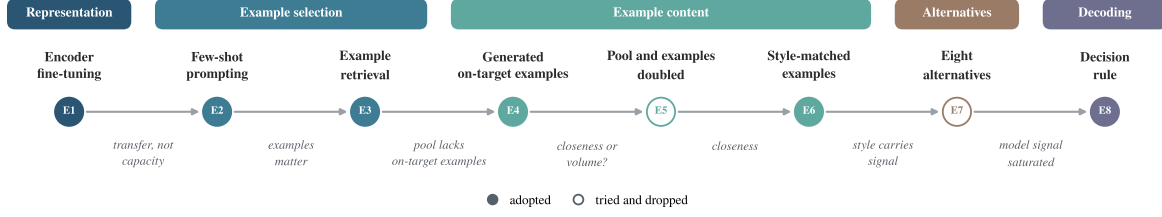
Figure 2: The eight experiments in the order they ran. The label under each arrow is the finding that led to the next step. Filled markers were adopted; hollow markers were dropped.
