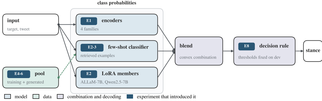
Figure 3: The system, with each component tagged by the experiment that introduced it: E1 encoders, E2 few-shot prompting and LoRA members, E3 retrieval, E4 to E6 the demonstration pool, E8 the decision rule. E7 added nothing: all eight of its experiments were dropped.
