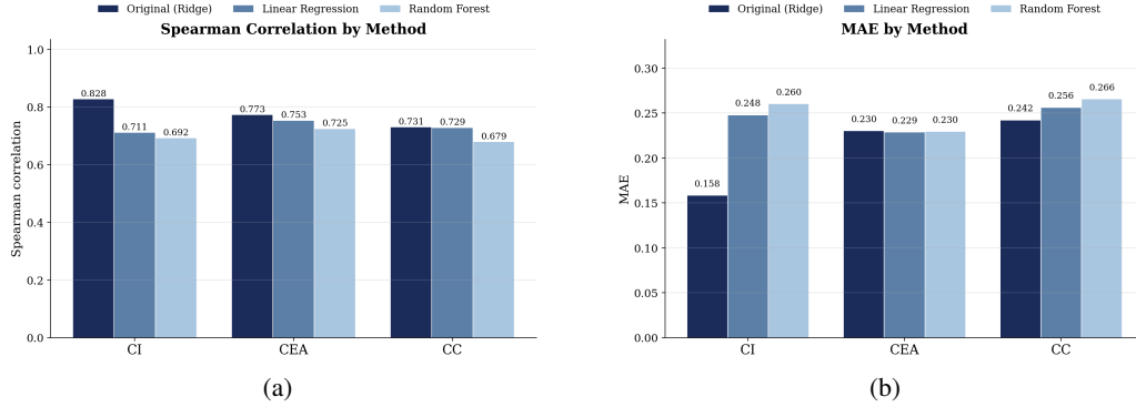
Figure 4: Comparison of the original score mapping with Linear Regression and Random Forest for CI, CEA, and CC: (a) Spearman correlation and (b) MAE on the development set.
