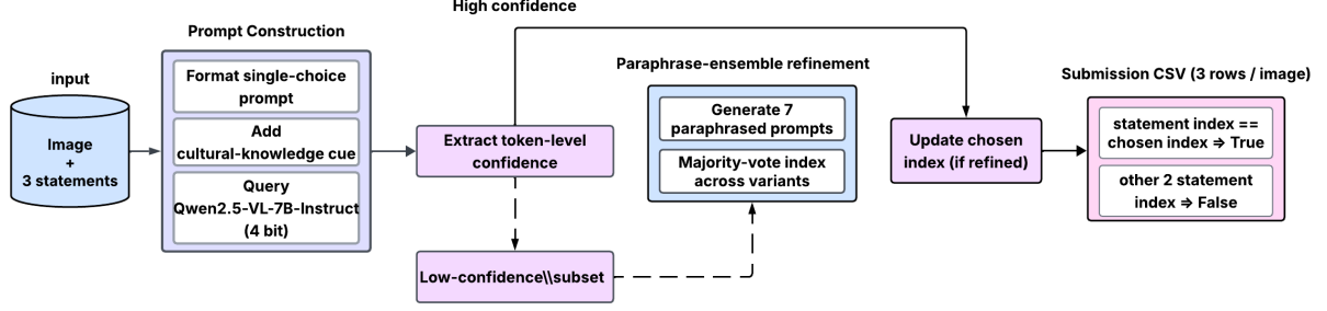
Figure 1: Proposed pipeline: single-choice VLM prompting, confidence-gated paraphrase-ensemble refinement for low-confidence items and expansion of the final index into per-statement True/False submission rows.
