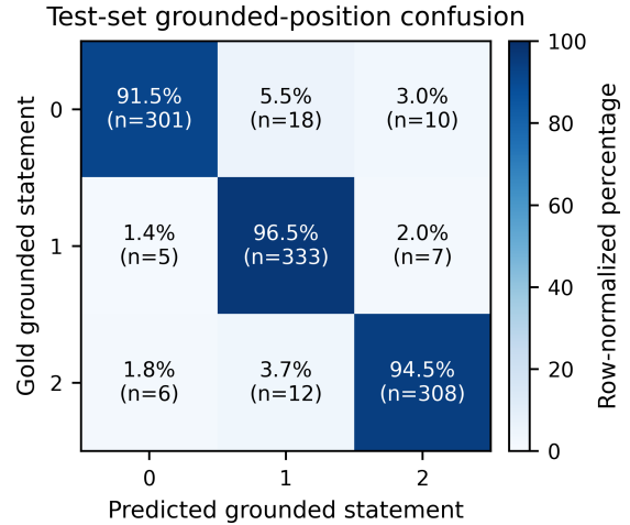
Figure 3: Confusion matrix of predicted grounded-statement position on the English test set, normalized by gold position, with raw counts in parentheses.
