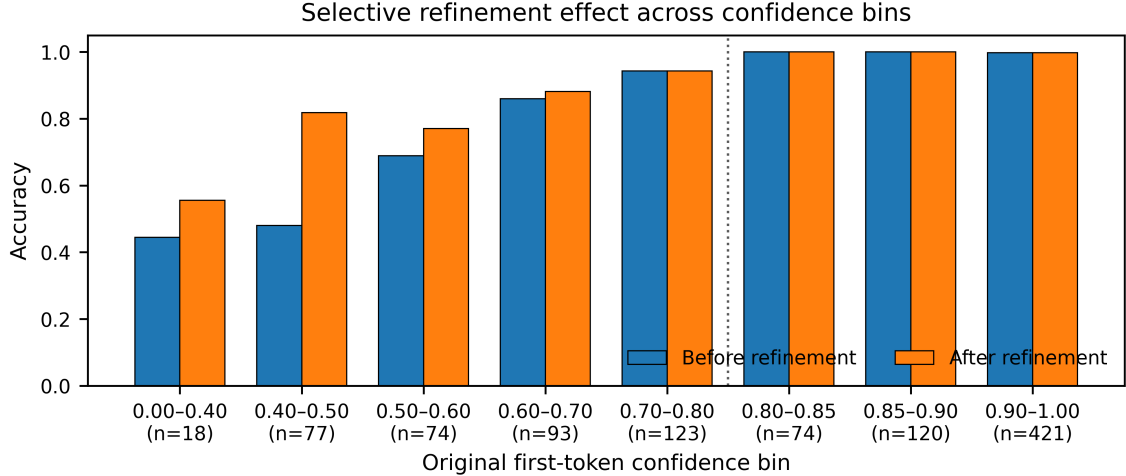
Figure 2: Effect of selective refinement across initial confidence bins on the English test set. Refinement has produced the largest gains for low-confidence predictions, with high-confidence predictions largely unchanged; values in parentheses indicate instance counts per bin.
