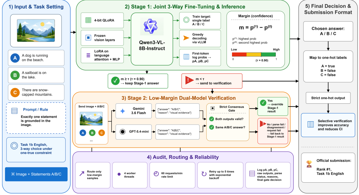
Figure 1: Overview of the submitted system. Stage 2 processes only low-margin items and changes the Stage 1 prediction only under strict agreement between the two verifiers.
