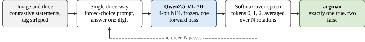
(a) Task 1b: one three-way forced choice, scored from option-token logits
