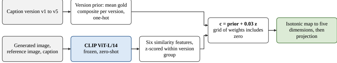
(b) Task 2: a six-parameter version prior with bounded CLIP tie-breaking
