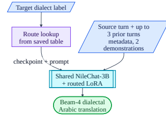
Figure 2: LahjaMT inference.
