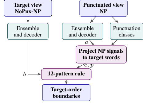
Figure 1: Two-view inference. The target decoder produces b ; the NP decoder produces a in NP token order. Projection maps a and NP punctuation to target-order signals e and p , which the rule combines with b .
