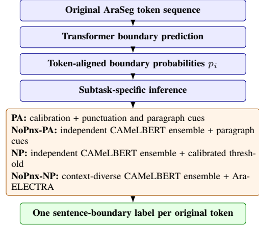
Figure 2: Wathiq-SPU AraSeg pipeline with subtask-specific inference strategies.
