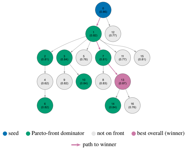
Figure 7: Full GEPA tree for the PA (Gemma) search: 17 candidates (candidate 13, path highlighted). Despite reaching the highest internal score of any PA LLM prompt this project produced, candidate 13 still lost to the manually improved prompt on the Blind Test set (Table 2).
