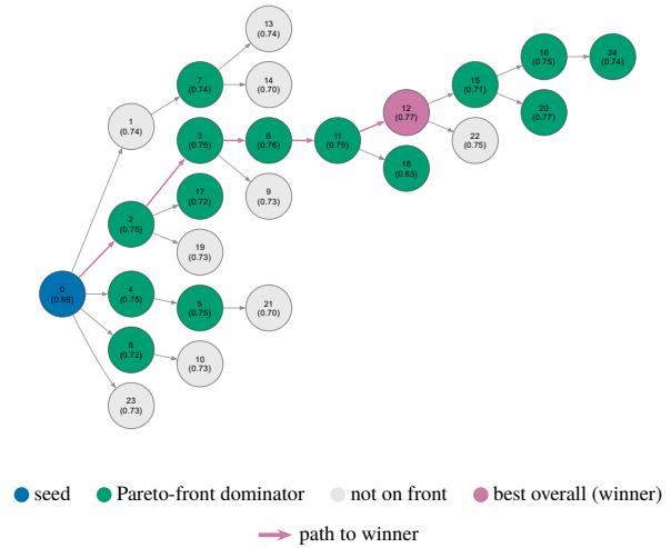
Figure 8: Full GEPA tree for the separate, later NoPnx-PA (Gemma) exploration: 25 candidates, own internal validation scale (see text). Candidate 12 is this run’s best; it was tested on the Blind Test set out of curiosity (a genuinely different prompt, worth trying on a stronger model) but no result from it is used anywhere in Table 2.
