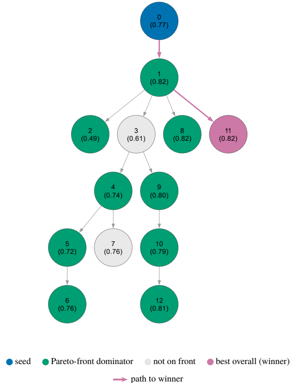
Figure 6: Full GEPA tree for the earlier NP (Gemma) search: 13 candidates, branching to depth 5, roles from the library’s own Pareto-front analysis (blue = seed, teal = Pareto-front dominator, gray = not on the front, purple = best overall/winner, path highlighted). Most candidates (teal), including several with a mediocre overall score like candidate 2 (0.4914), are still Pareto-front dominators – each is the single best candidate on at least one validation example, which is exactly why GEPA keeps exploring from them instead of only from the current overall best.
