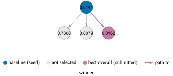
Figure 5: NoPnx-NP GEPA meta-harness tree: baseline (blue) branches into three iteration-2 mutations, two of which regress (gray) and one of which is submitted (purple, path highlighted) – oversplit_then_merge (−0.0273), gap_audit_verification (−0.0062), hierarchical_coarse_to_fine (+0.0022, submitted; full names in Table 9). No per-example Pareto-front data exists for this engine, so unlike the trees below, gray here means simply “not selected,” not “off the front.”
