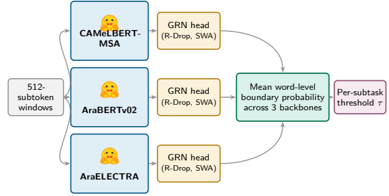
Figure 1: Supervised 3-backbone ensemble (Section 3.1): each backbone is fitted independently with a Gated Residual Network head, trained with R-Drop and stochastic weight averaging; the three backbones’ word-level boundary probabilities are averaged and thresholded per subtask.
