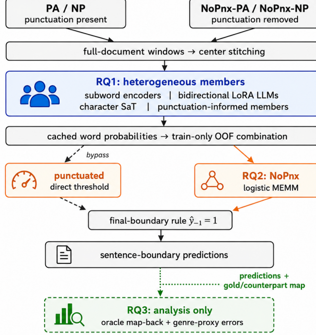
Figure 1: Production inference and post-hoc analysis. Punctuated systems bypass the MEMM; only punctuation-free systems take the amber decoding branch. The green dotted branch uses predictions and gold-aligned counterparts for analysis and is never part of inference. Labels and line styles preserve meaning in grayscale.
