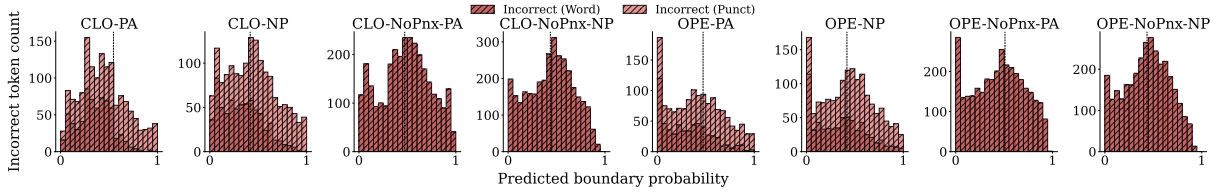
Figure 2: Confidence distribution of incorrect predictions, split into word tokens and punctuation tokens, across closed and open tracks for all four signal conditions. Punctuation-token errors are hatched to distinguish them from word-token errors. Token counts are shown on a linear scale.
