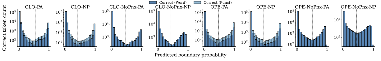
Figure 1: Confidence distribution of correct predictions, split into word tokens and punctuation tokens, across closed and open tracks for all four sub-tasks. Token counts are shown on a log scale due to class imbalance.
