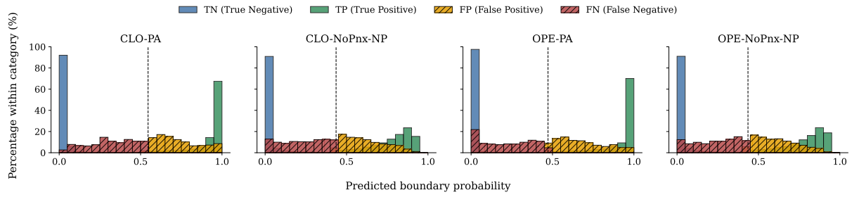
Figure 3: Per-category confidence distributions (TN, TP, FP, FN, each normalized to 100% within its own category) for the full-signal (PA) and fully-stripped (NoPnx-NP) conditions, across closed and open tracks. Contrasting these two endpoint conditions highlights the cumulative effect of removing both punctuation and paragraph markers.
