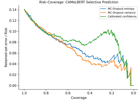
Figure 2: Selective risk-coverage for CAMELBER. Lower retained-set risk is better as uncertain cases are deferred.
