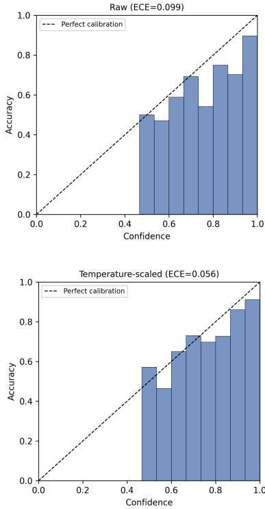
Figure 1: CAMELBER reliability diagrams before and after temperature scaling.
