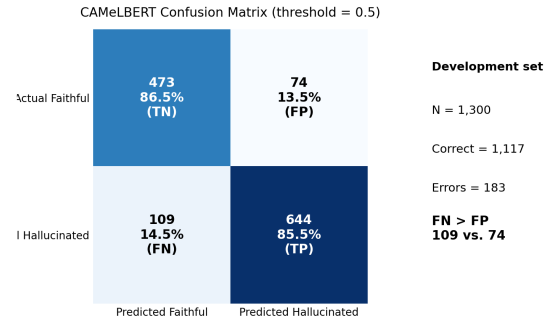
Figure 3: CAMELBER development confusion matrix at threshold 0.5: 473 TN, 74 FP, 109 FN, and 644 TP. False negatives are more frequent than false positives at this operating point.
