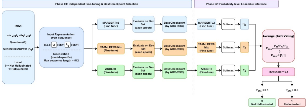
Figure 1: Overview of the proposed ensemble framework for Arabic hallucination detection.
