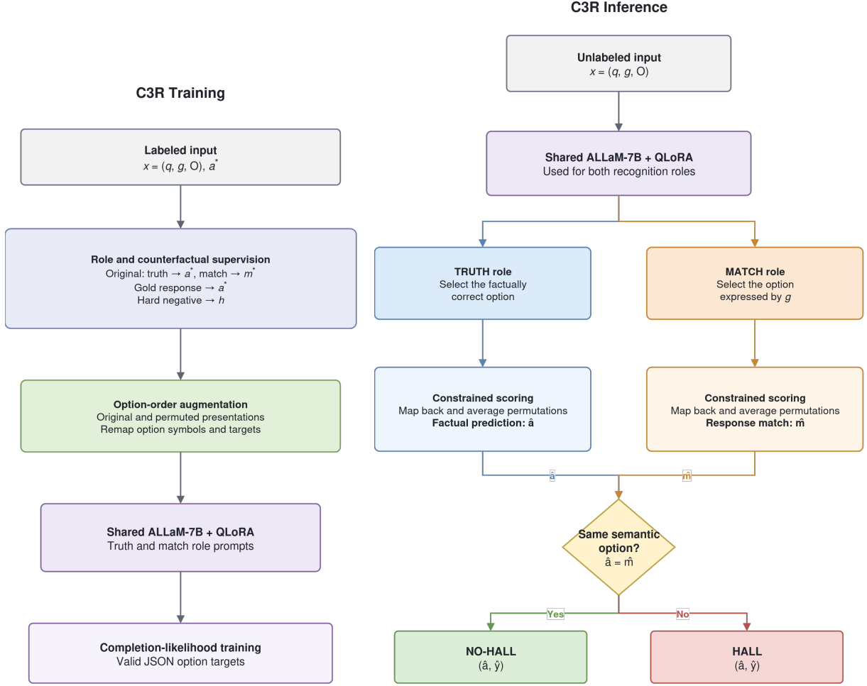
Figure 1: Separate C3R pipelines for counterfactual training (left) and cross-role inference (right).
