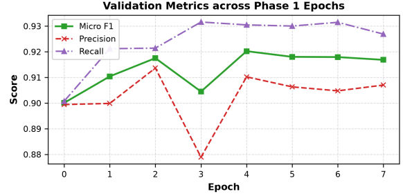
Figure 1: Validation Micro F1, Precision, and Recall metrics over Phase 1 (supervised training) epochs on the Wojood validation set (Seed 42).
