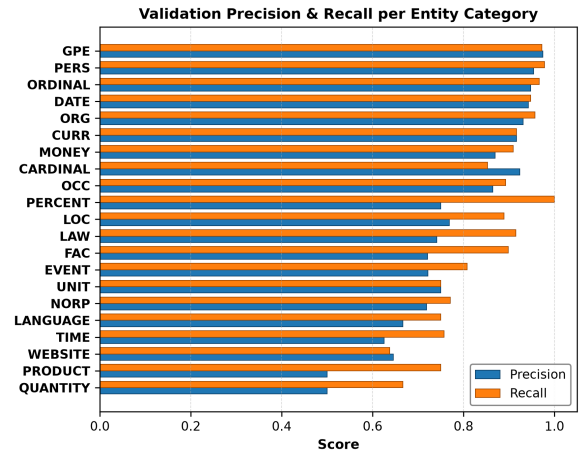
Figure 2: Per-category validation Precision and Recall on the Wojood validation set (evaluated on the post-adaptation SWA model).
