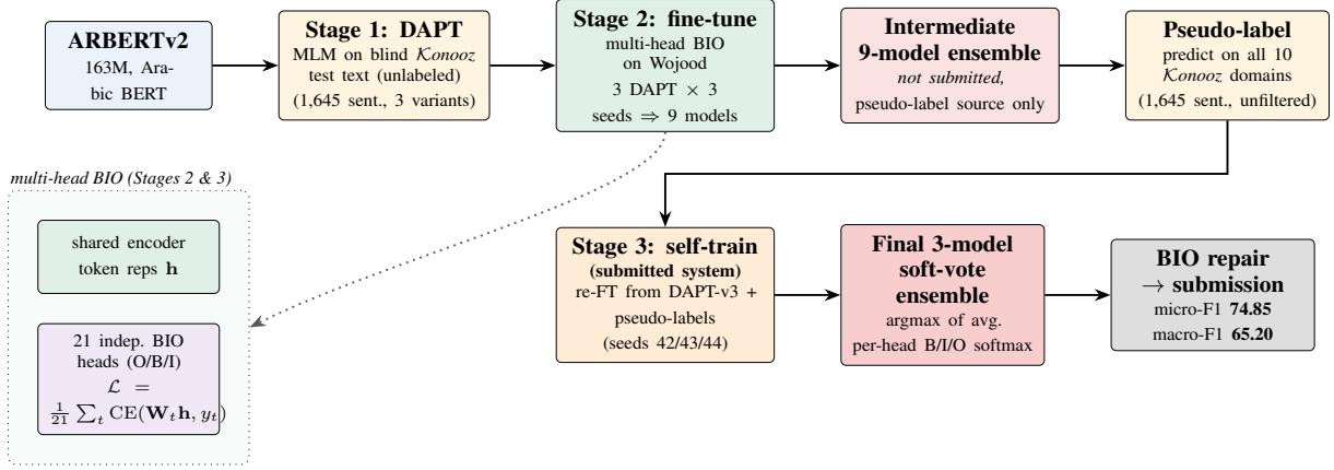
Figure 1: Our NER pipeline. DAPT adapts ARBERTv2 to the unlabeled Konooz text. The resulting encoders are fine-tuned with a multi-head BIO architecture on Wojood. Self-training then re-fine-tunes three new seeds from the DAPT-v3 checkpoint on Wojood plus pseudo-labels produced by the intermediate 9-model ensemble. Stage 1 and the pseudo-labeling step both consume the blind Konooz test sentences (without labels), making the pipeline transductive (§4.1).
