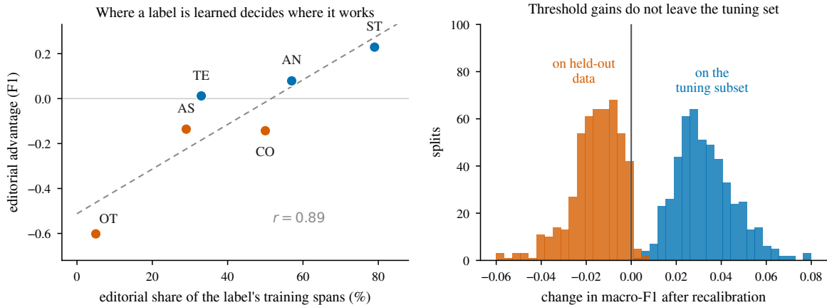
Figure 5: The two post-submission findings. Left, each label’s editorial advantage on the development set against the editorial share of that label’s training spans, with OT at the extreme and the dashed line a least-squares fit. Right, the change in Task 1 macro-F1 after recalibrating per-class thresholds on a quarter of the out-of-fold paragraphs, measured on the tuning subset and on the held-out remainder over 500 random splits. The in-sample distribution lies entirely above zero, while the held-out distribution is non-positive in 97% of splits.
