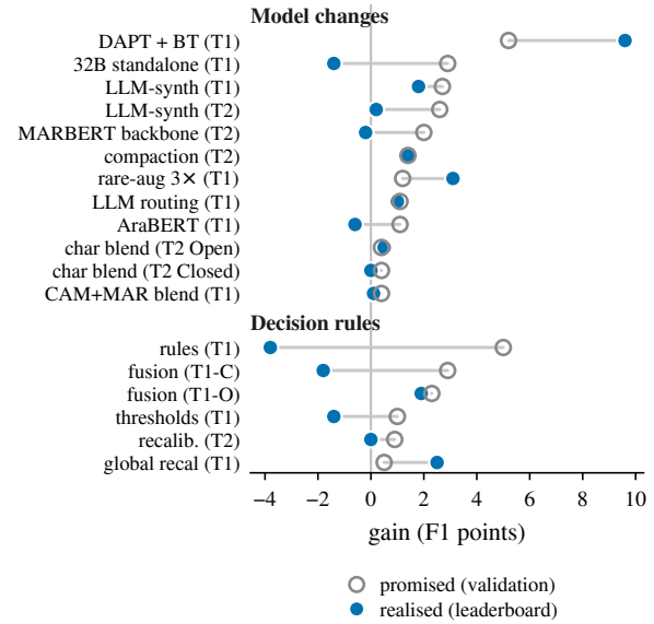
Figure 4: Promised validation gain (open) and realised leaderboard gain (filled) for the eighteen interventions, in F1 points, sorted by promise. Labels are abbreviated forms of the row names in Table 6, where the full data appear.
