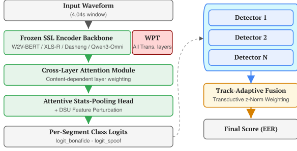
Figure 1: System architecture: per-detector scoring followed by track-adaptive late fusion.
