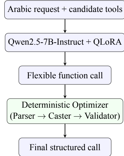
Figure 1: Overview of our Generative-Optimizer pipeline.
