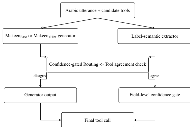
Figure 7: Overview of the Makeeen pipeline. The submitted Makeeen Base generator is extended with label-semantic extraction for Makeeen +Hint and with confidence-gated routing at inference time.
