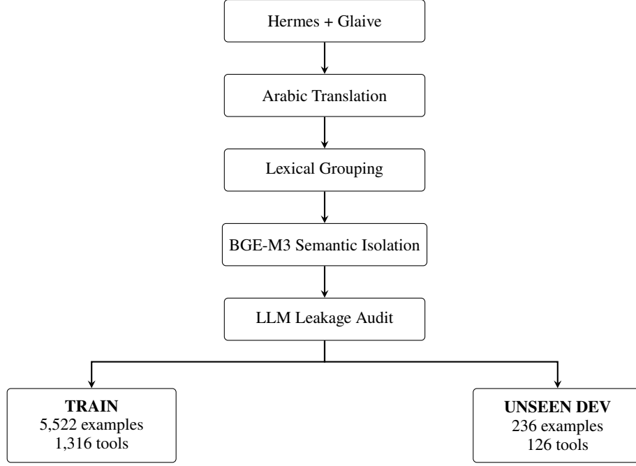
Figure 6: Construction of the external-tool training and unseen-tool development sets. Hermes and Glaive examples are translated into Arabic, grouped lexically, filtered using BGE-M3 semantic similarity to isolate tool groups, and subsequently audited with an LLM to reduce potential cross-split leakage. The final split is performed at the tool level, with 1,316 training tools and 126 unseen development tools.
