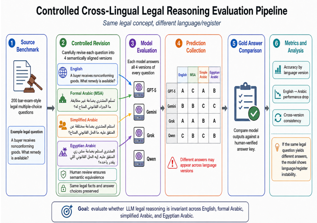
Figure 1: Controlled evaluation pipeline for legal reasoning across English and three Arabic language varieties.
