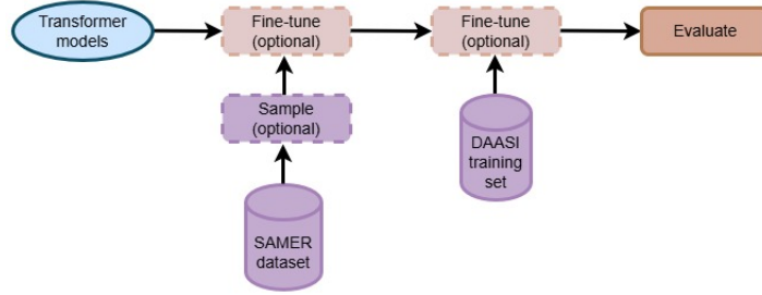
Figure 2: Evaluation pipeline.
