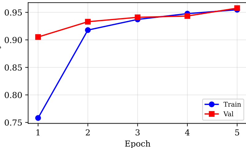
Training / Validation Accuracy
