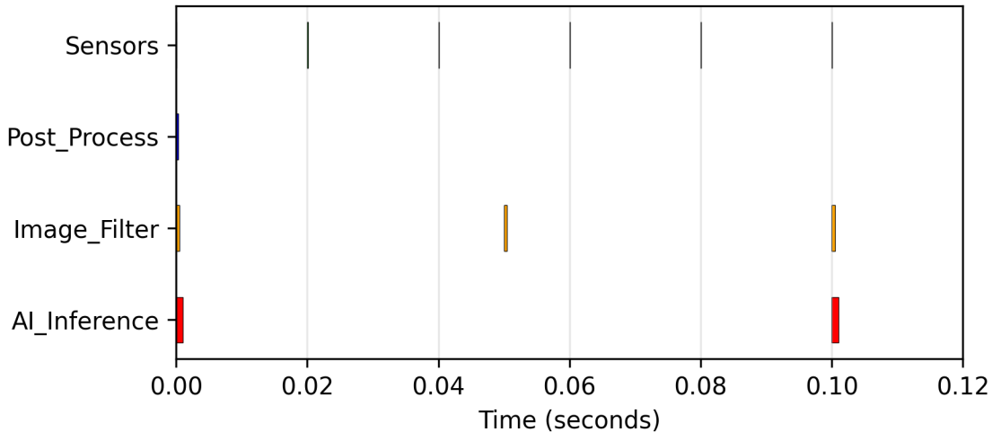
FreeRTOS RMS Schedule ( U=0.027 \leq 0.757 )
