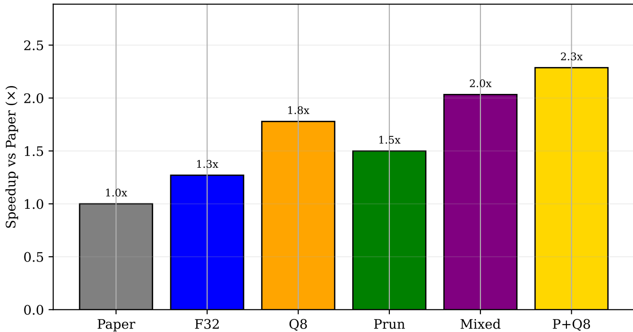
Throughput Speedup over Paper Baseline
