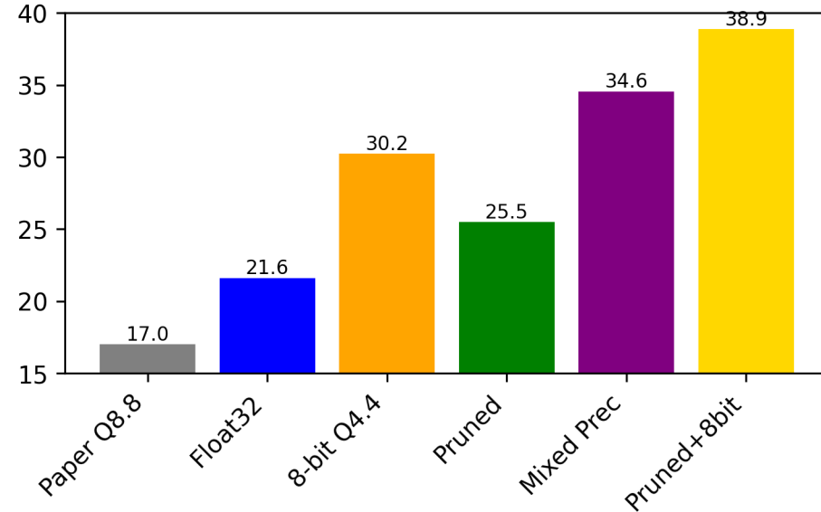
ZedBoard FPS
