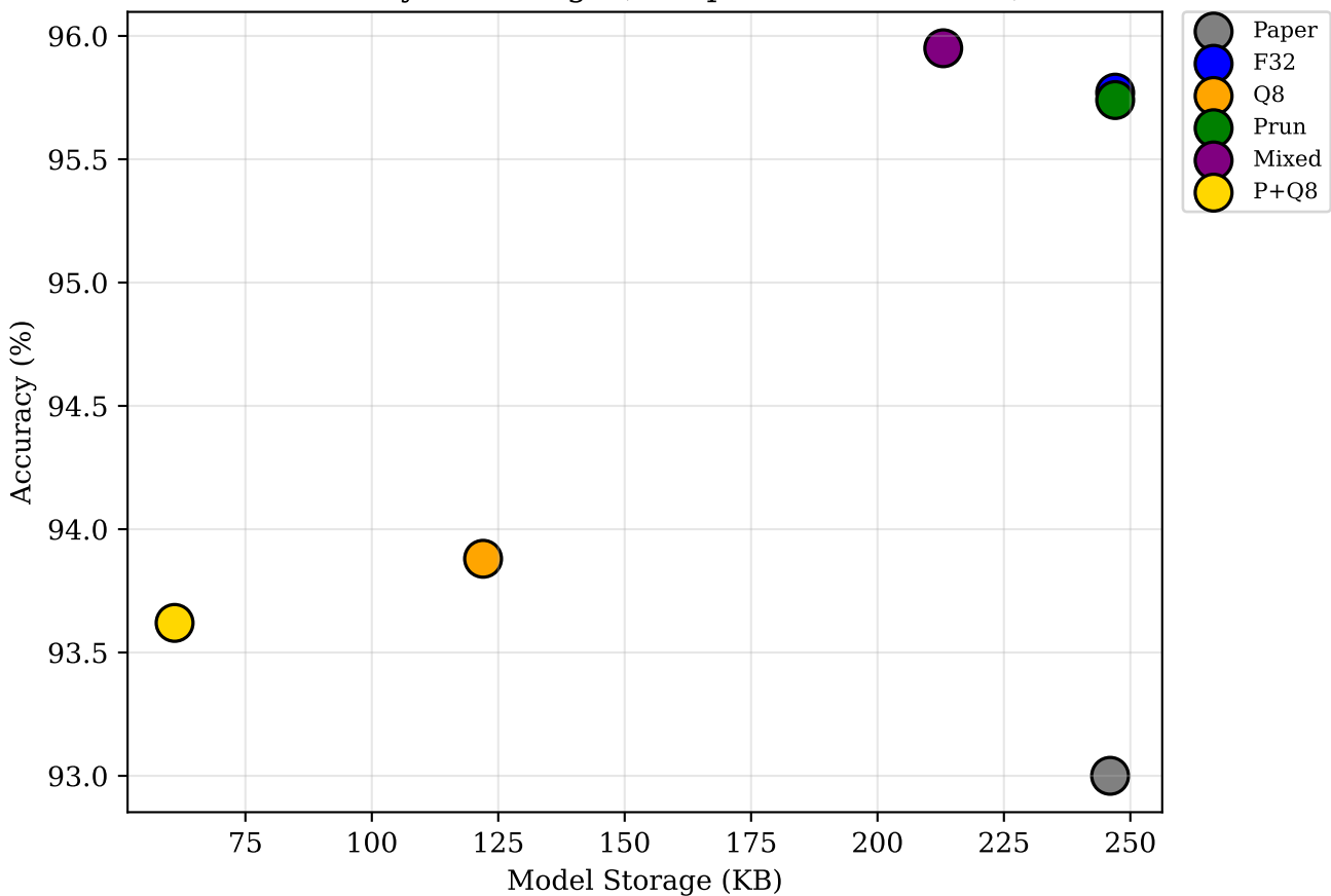
Accuracy vs Storage (Compression Trade-off)
