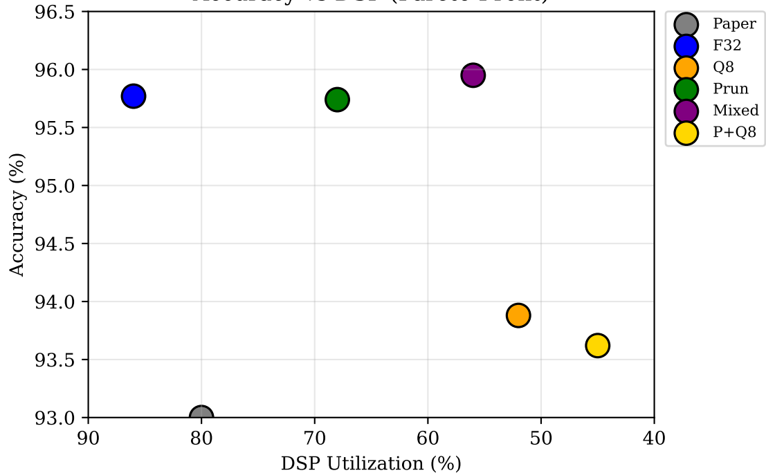
Accuracy vs DSP (Pareto Front)
