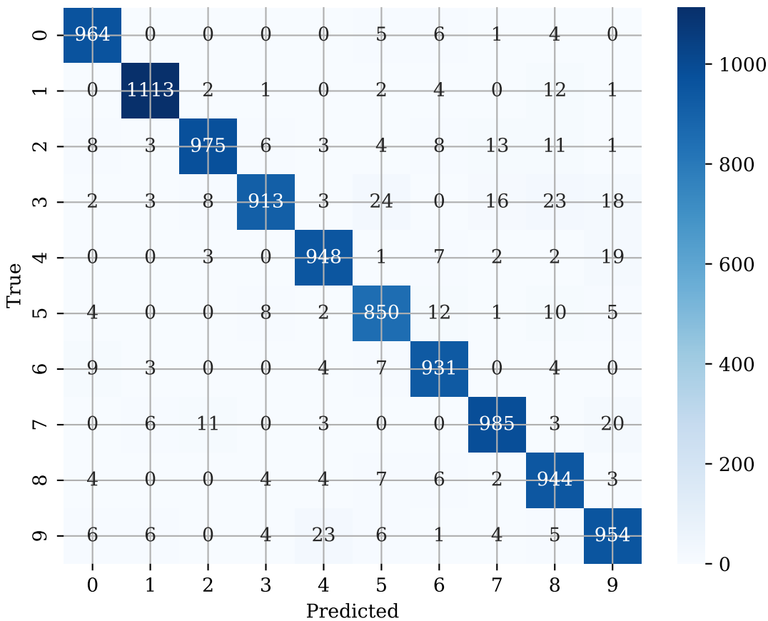
LeNet-5 Confusion Matrix (MNIST)
