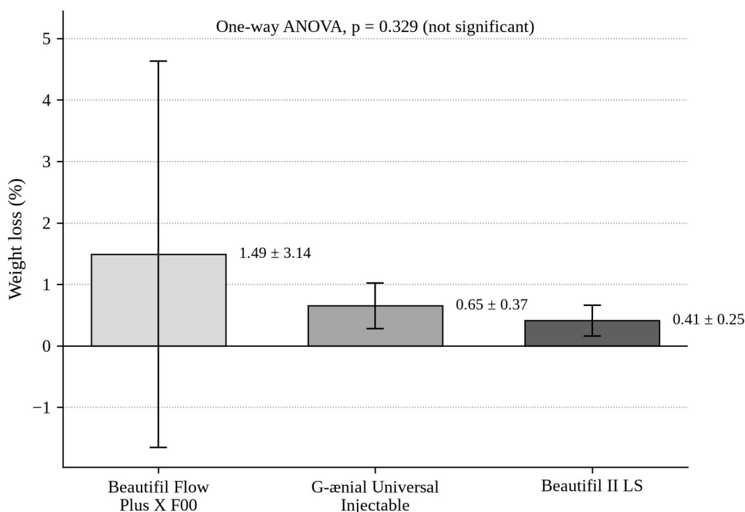
Figure 4.1 Mean percentage weight loss of the three composite resins after 10 000 toothbrushing cycles at 2 N. Error bars represent one standard deviation ( n = 12 per group). In the Beautifil Flow Plus X F00 group the standard deviation exceeds the mean, so the lower error bar extends below zero; this reflects the dispersion introduced by a single specimen that lost approximately 11.4 % of its mass and does not imply a gain in weight. Differences among groups were not statistically significant (one-way ANOVA, p = 0.329 ).
