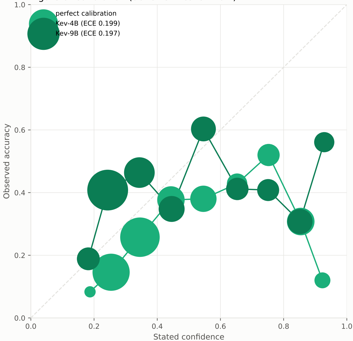
Figure 6. Calibration (dot size = calls in bin)
