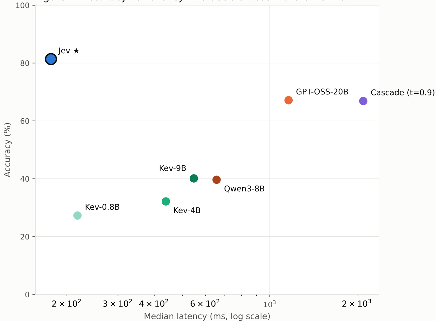
Figure 1. Accuracy vs. latency: the decision-cost Pareto frontier
