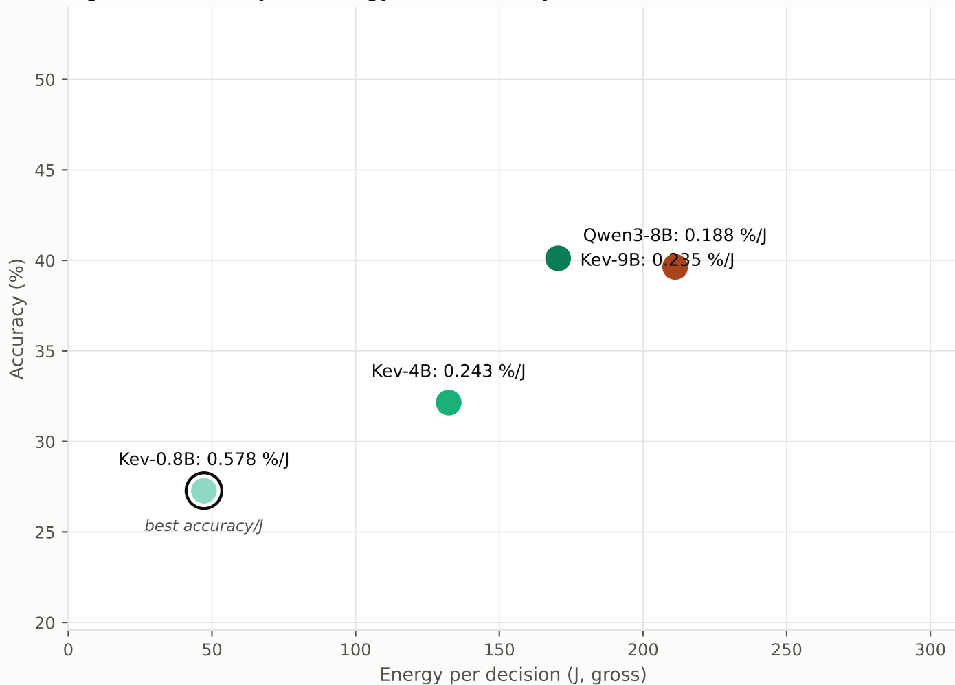
Figure 4. Accuracy vs. energy: the efficiency frontier
