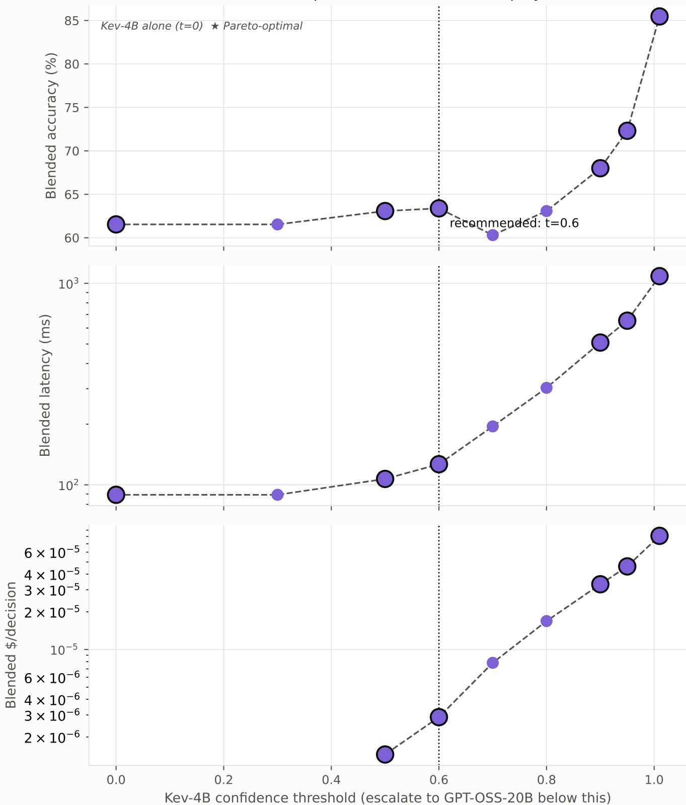
Cascade accuracy / latency / cost vs. confidence threshold (outlined markers = Pareto-optimal; simulated from replayed calls)
