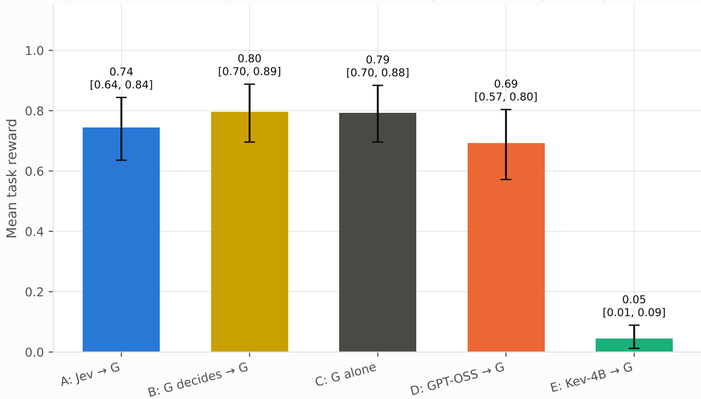
Figure 11. Task reward per arm, 95% CI clustered by task ( \geq 244 episodes per arm)
