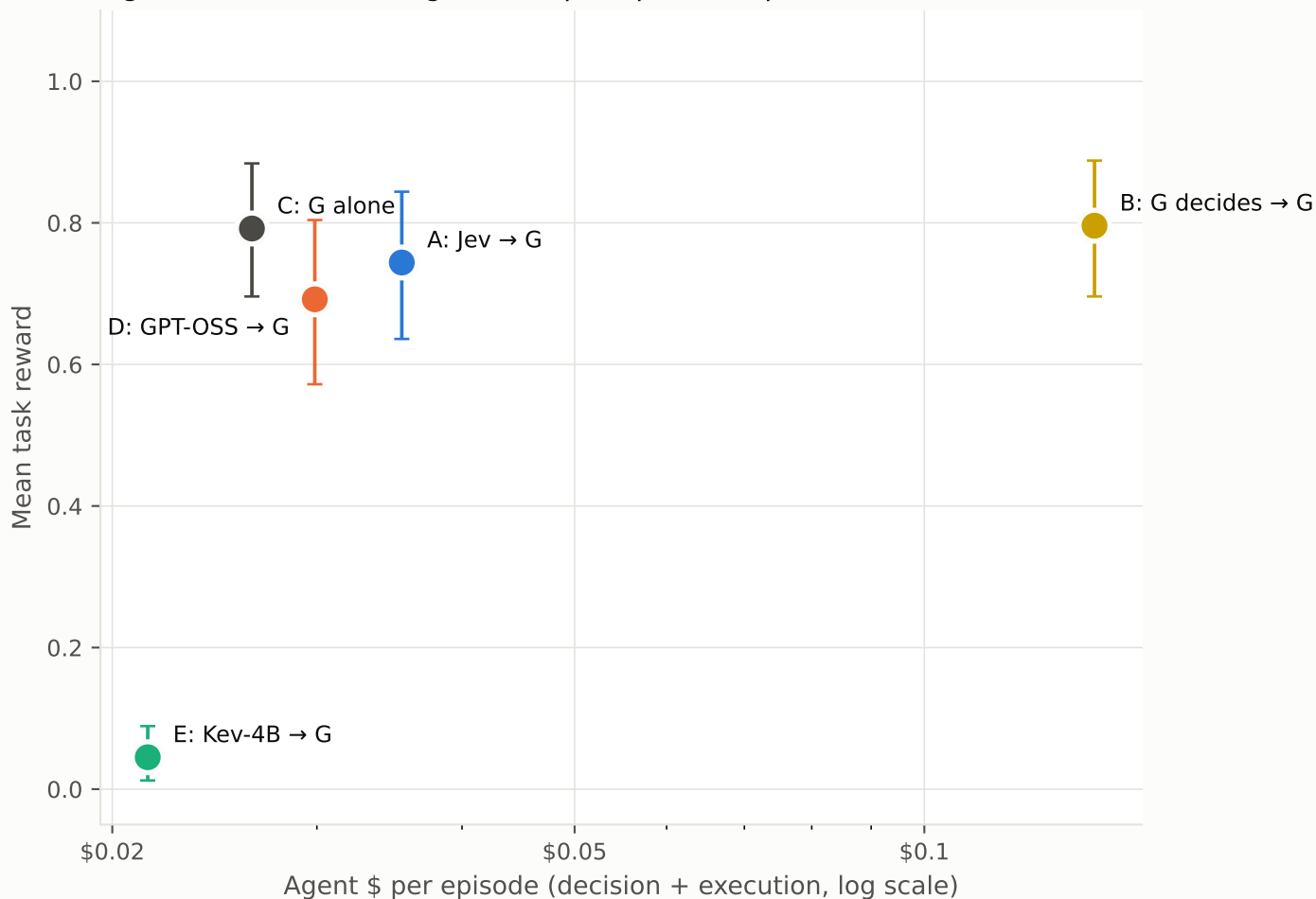
Figure 12. Reward vs. agent cost per episode (up-left is better)
