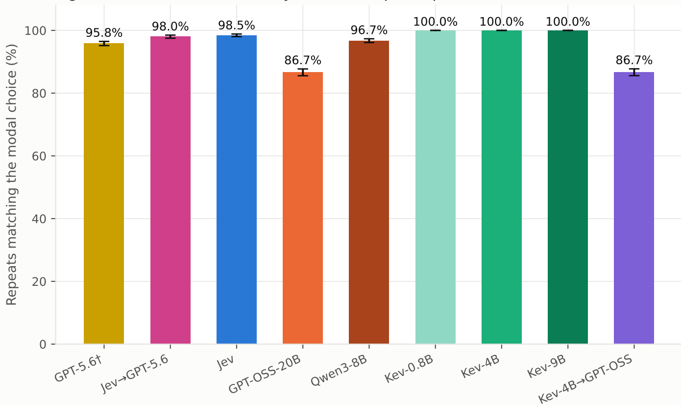
Figure 5. Decision consistency across 5 repeats per state
