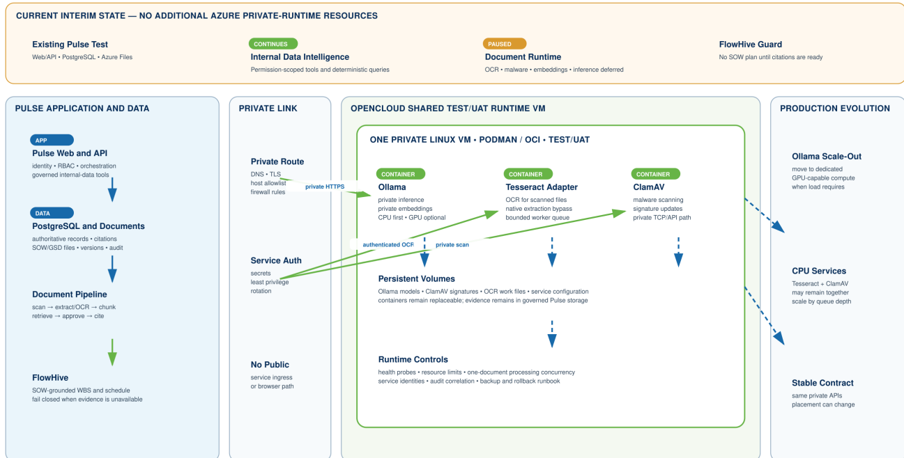
Figure 3. OpenCloud shared private-runtime VM for Ollama, Tesseract, and ClamAV in Test/UAT.
