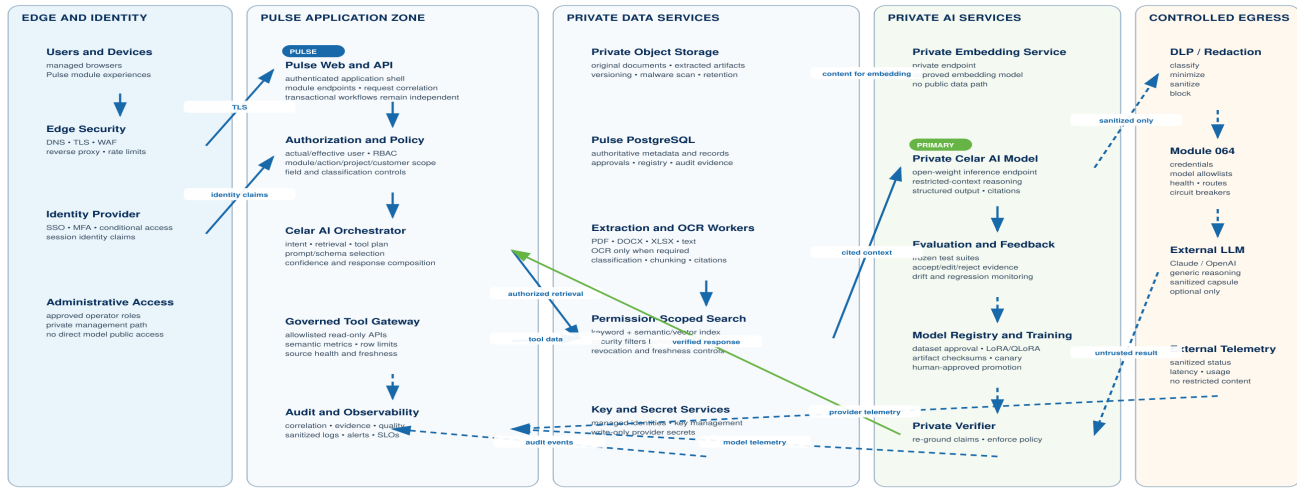
Figure 2. Celar AI deployment and network architecture.
