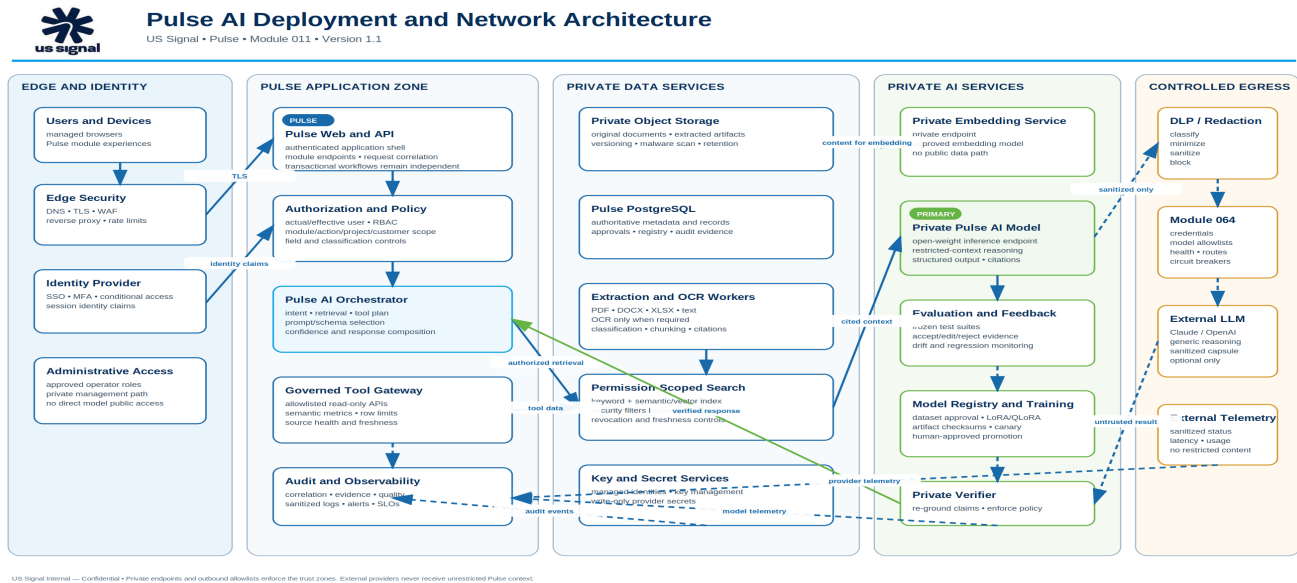
Figure 2. Pulse AI deployment and network architecture.
