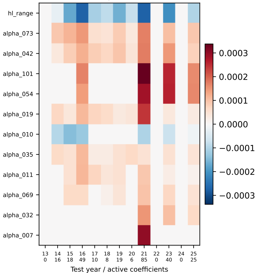
1-day horizon
