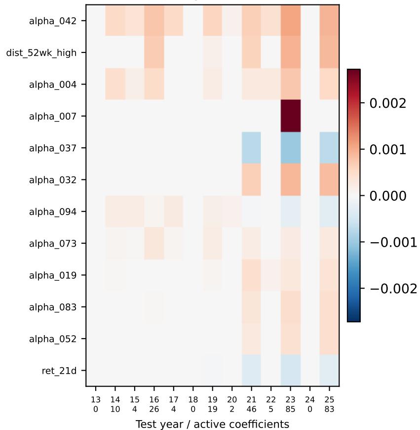
5-day horizon
