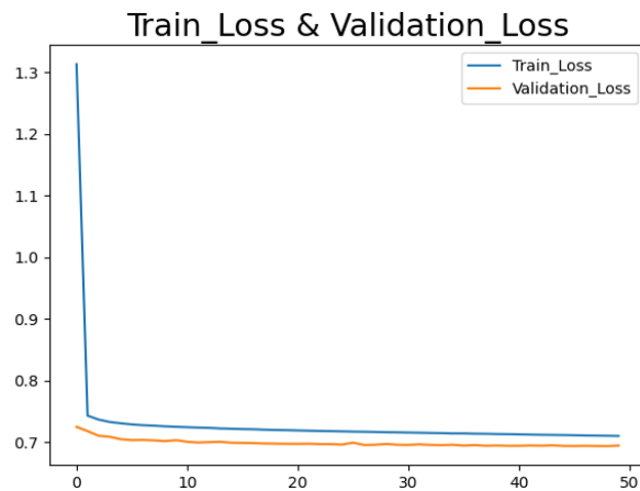
Figure (46) Training the Autoencoder
