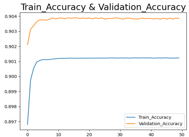
Figure (46) Training the Autoencoder
