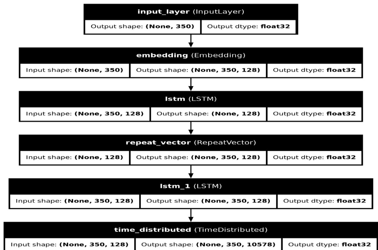
Figure (45) Autoencoder Block
