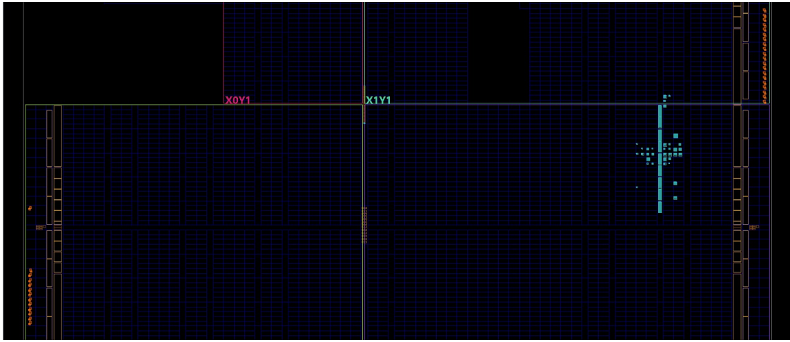
Figure 19: Post-implementation device placement view for the routed baseline.
