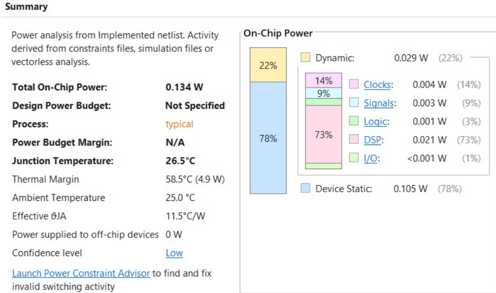
Figure 24: Vivado power-report evidence for the current routed baseline.
