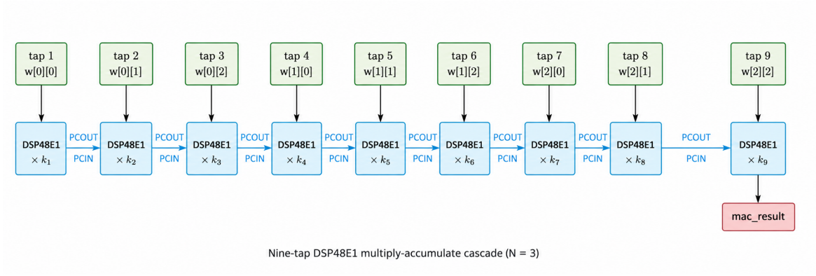
Figure 18: The accumulator cascade lives inside the DSP columns: each stage adds the incoming cascade into its own product. Moving accumulation into fabric would cost \sim 20 LUTs per stage.
