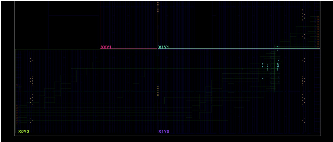
Figure 20: Post-implementation routed device view for the routed baseline.
