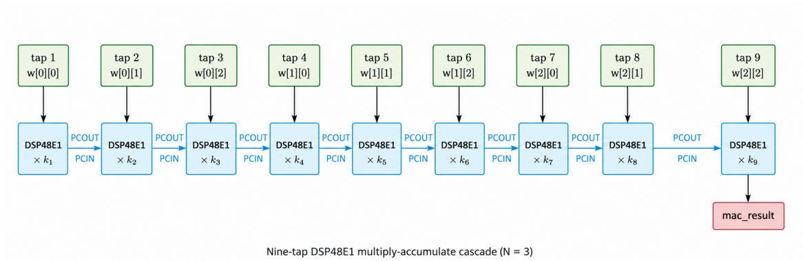
Figure 21: The accumulator cascade lives inside the DSP columns: each stage adds the incoming cascade into its own product. Moving accumulation into fabric would cost \sim 20 LUTs per stage.
