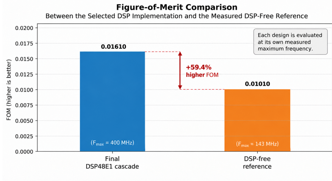
Figure 31: Figure-of-merit comparison between the selected DSP implementation and the measured DSP-free reference.
