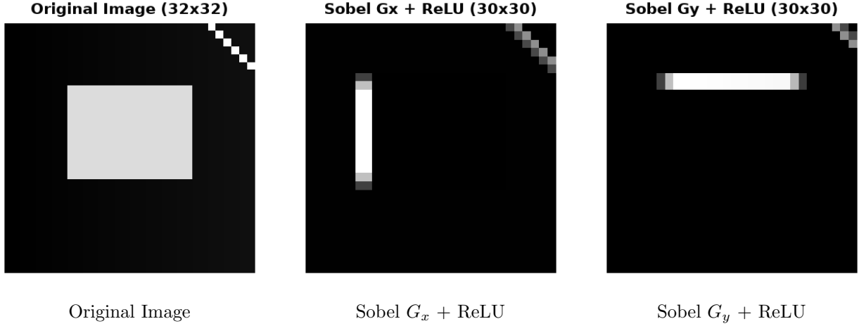
Figure 14: Hardware edge-detection demonstration using runtime-programmed Sobel operators. The 30 \times 30 valid outputs natively isolate vertical ( G_x ) and horizontal ( G_y ) edges. The ReLU stage cleanly zeros out negative gradients, validating the output conditioning logic.
