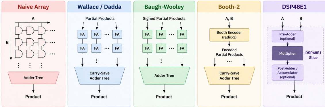
Figure 15: Visual comparison of the multiplier architectures considered during the design-space exploration.
