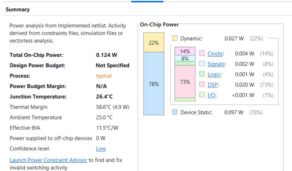
Figure 27: Vivado power-report evidence for the current routed baseline before SAIF annotation.
