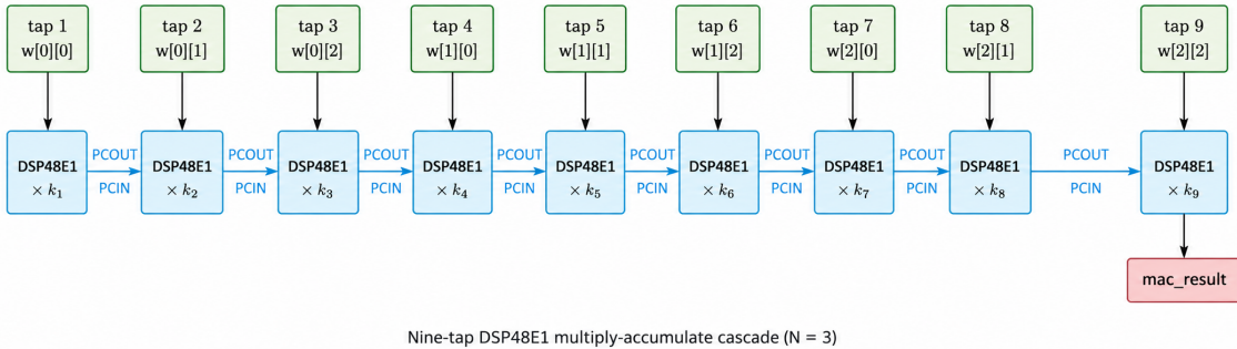
Figure 21: The accumulator cascade lives inside the DSP columns: each stage adds the incoming cascade into its own product. Moving accumulation into fabric would cost \sim 20 LUTs per stage.
