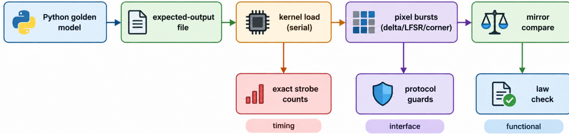
Figure 8: Testbench flow: golden generation feeds the file-comparison layer; stimulus and independent checks run per burst.
