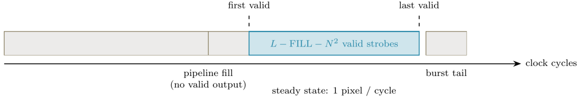
Figure 7: Streaming timing of one burst. For N=3 , W=32 , L=1100 : FILL = 66 , accumulation pipeline = 9, valid strobes = 1025.
