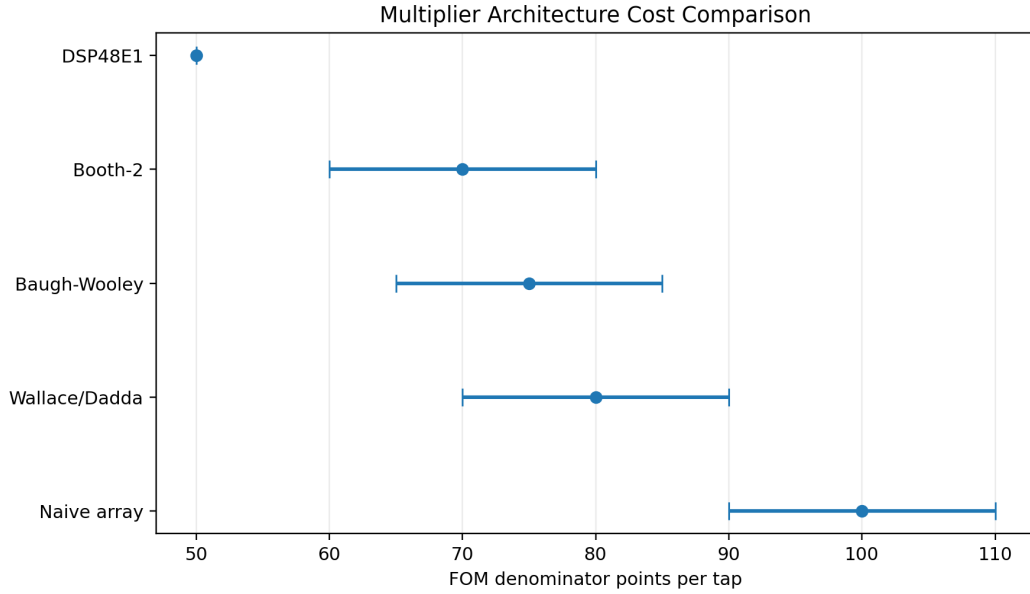
Figure 14: Multiplier decision study. Fabric techniques are shown as their estimated per-tap FOM-denominator cost ranges; the DSP48E1 point is the exact 50-point competition price. The final DSP choice was then confirmed by a measured DSP-free implementation.
