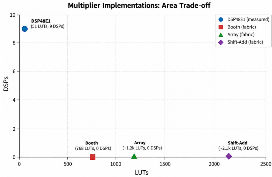
Figure 16: Architecture comparison illustrating DSP48E1-based multiplication and accumulation versus the fabric multiplier/accumulator alternative.
