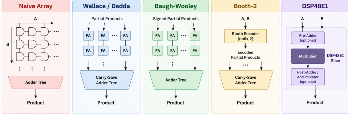
Figure 13: Visual comparison of the multiplier architectures considered during the design-space exploration.
