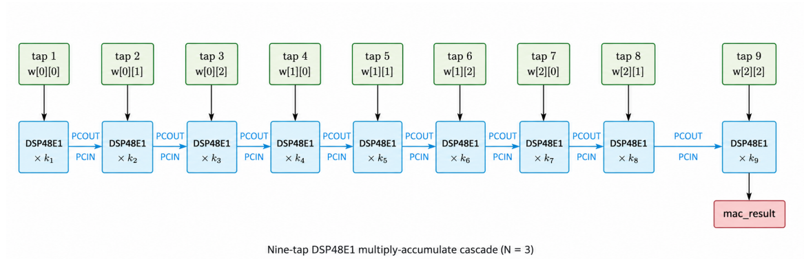
Figure 19: The accumulator cascade lives inside the DSP columns: each stage adds the incoming cascade into its own product. Moving accumulation into fabric would cost \sim 20 LUTs per stage.
