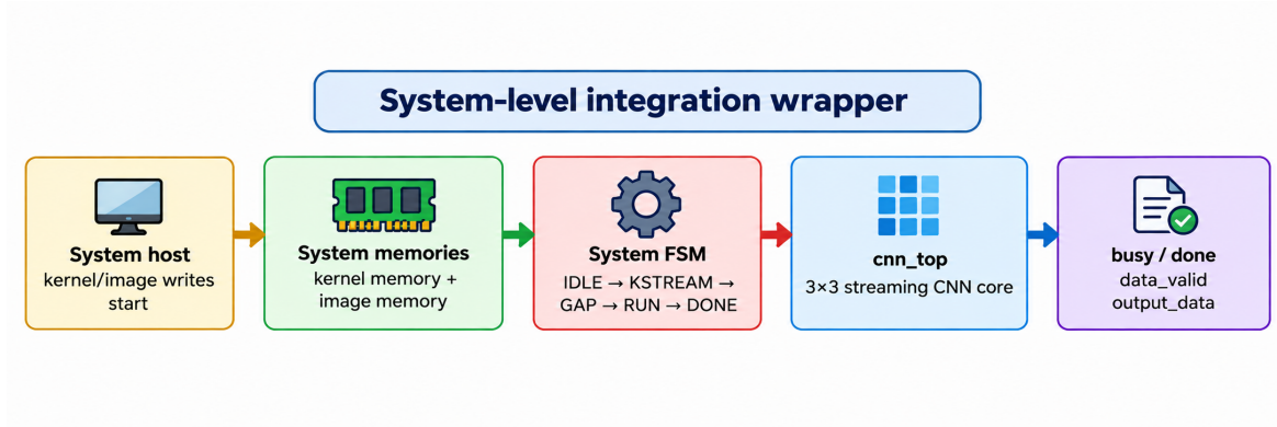
Figure 11: System-level wrapper used for integration verification. Local memories hold the kernel and input stream; the wrapper FSM feeds them to the existing CNN core and exposes simple host-side start / busy / done signals.
