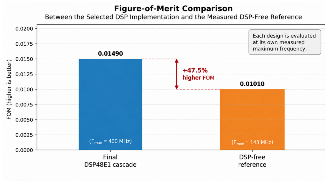
Figure 26: Figure-of-merit comparison between the selected DSP implementation and the measured DSP-free reference.
