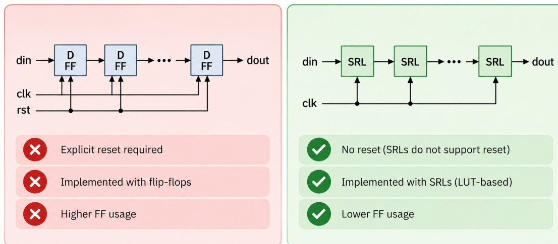
Figure 17: Storage mapping comparison showing SRL-based versus flip-flop-based implementations of the line buffers and tap delays.
