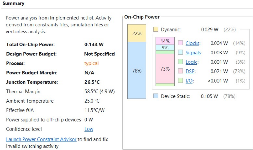
Figure 25: Vivado power-report evidence for the current routed baseline.
