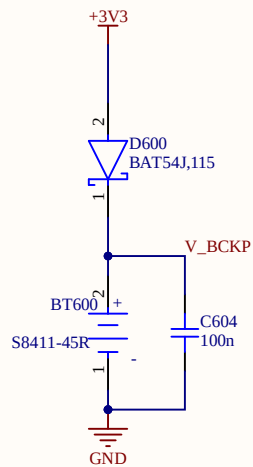
Back up Battery
