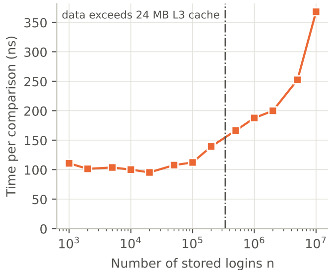
Cost of one comparison
