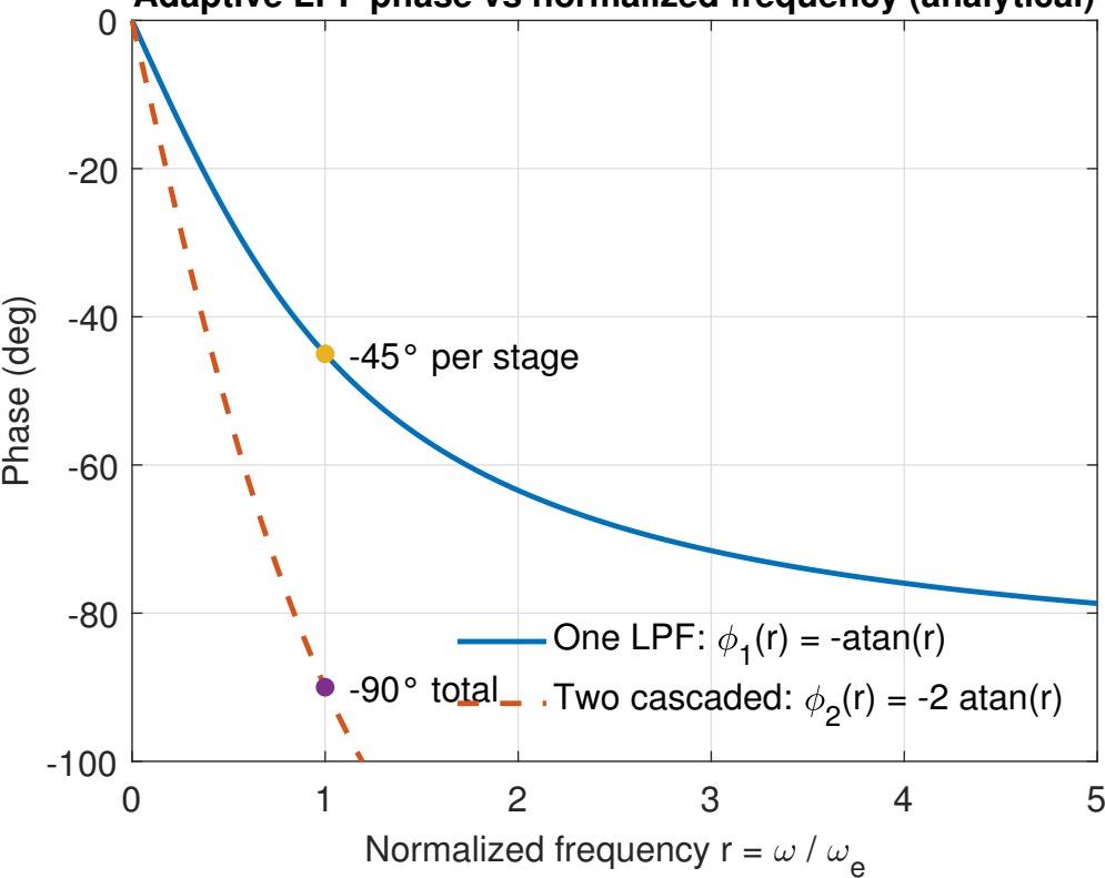
Adaptive LPF phase vs normalized frequency (analytical)
