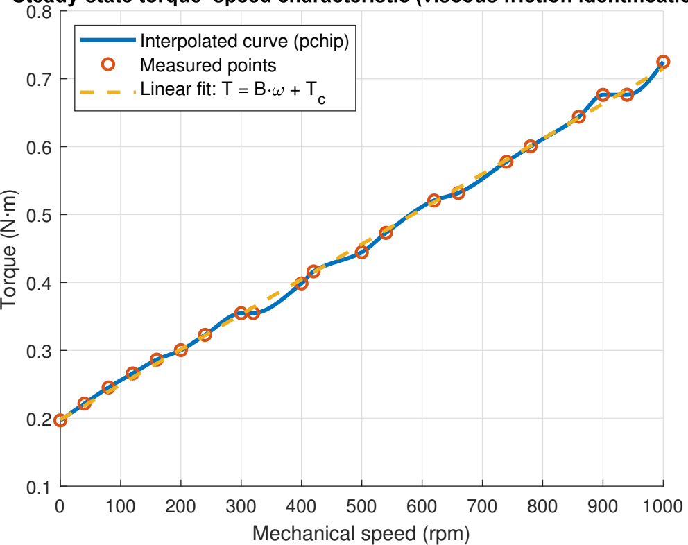
Steady-state torque–speed characteristic (viscous friction identification)
