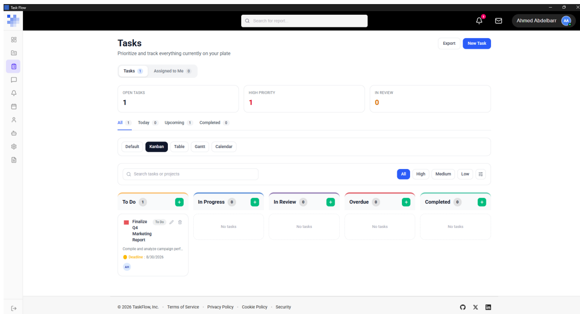
Figure 3.3: Kanban view of the Tasks module with five colour-coded status columns and drag-and-drop support.
