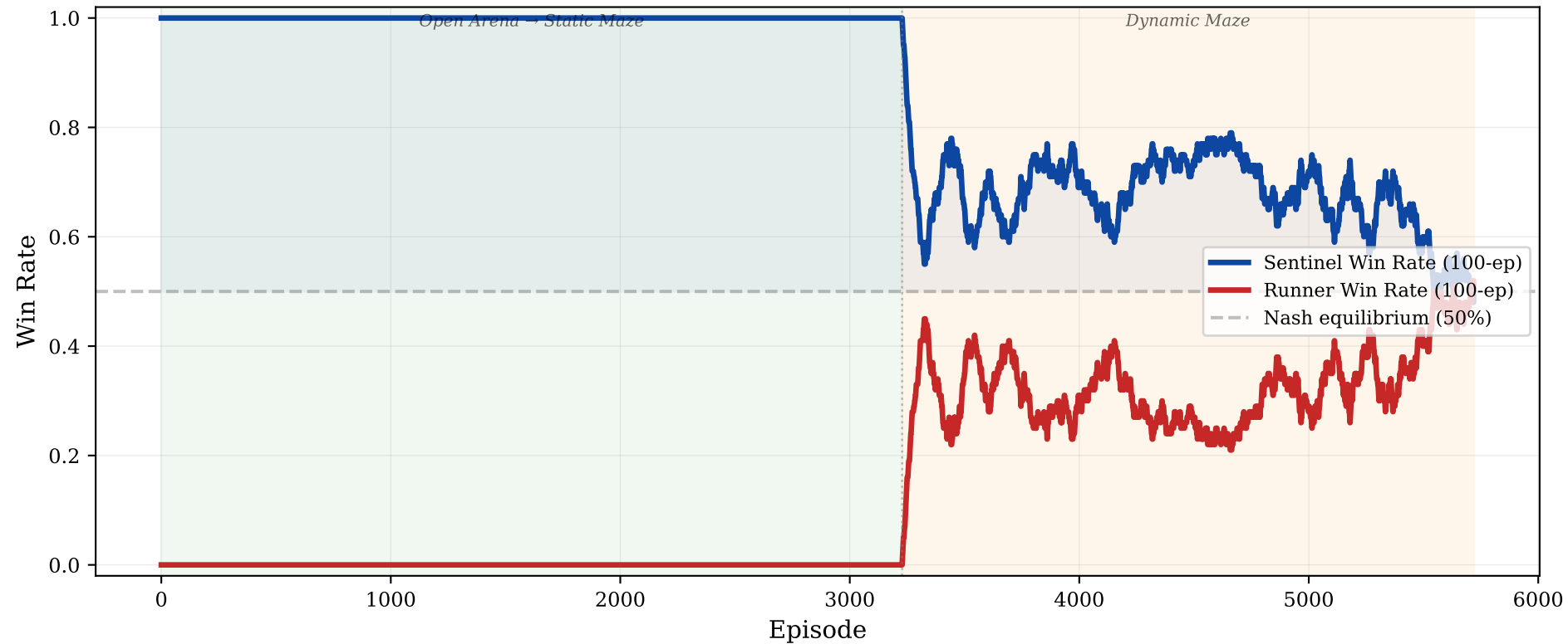
Win Rate Convergence Across Curriculum Phases
