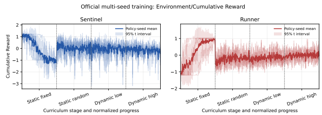
Fig. 4. Audited five-seed official curriculum reward curves exported from TensorBoard scalars. The official gate uses fixed trainer step budgets. The plotted curves are diagnostic summaries of completed training.
