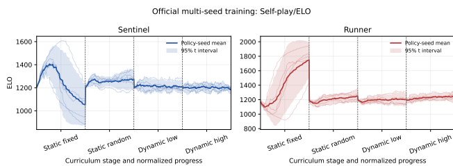
Fig. 5. Audited five-seed self-play ELO traces. Stable or increasing ELO does not imply Nash convergence. It is used as a training diagnostic.
