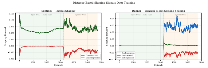
Fig. 10. Archived shaping traces motivating the tactical-reward extension.
