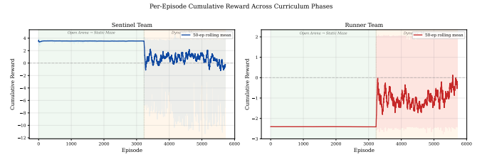
Fig. 6. Excluded legacy three-phase cumulative reward. Not comparable to the official v5 curriculum.
